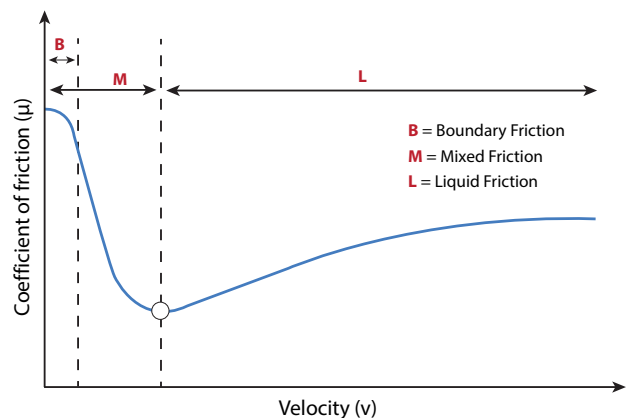
Friction Conditions Prevailing Inside the Cylinder
